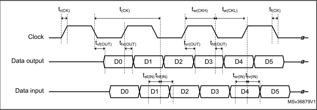
Figure 71. DDR mode
