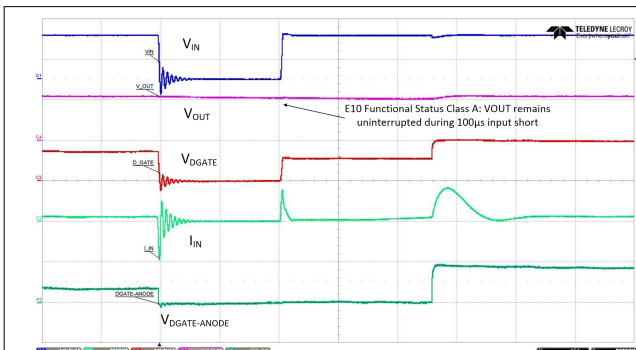
Figure 10-5. Input Micro-Short - LV124 E10 TC 2 100 \mu s
