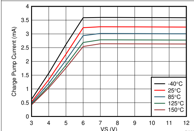
Figure 7-3. Charge Pump Current vs Supply Voltage at CAP = 6 V
