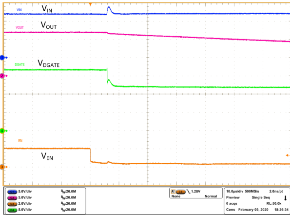
Figure 10-21. Turn OFF Delay - DGATE
