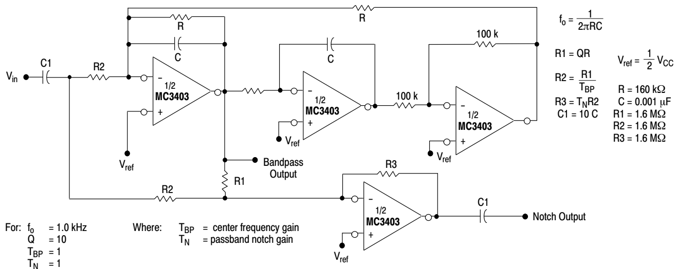
Figure 13. Bi-Quad Filter
