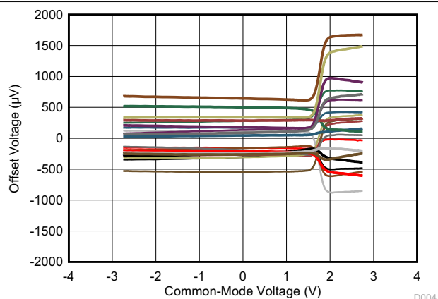
Figure 7-4. Offset Voltage vs Common-Mode
