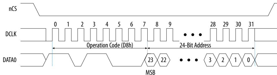
Figure 20. Erase Sector Operation Timing Diagram
