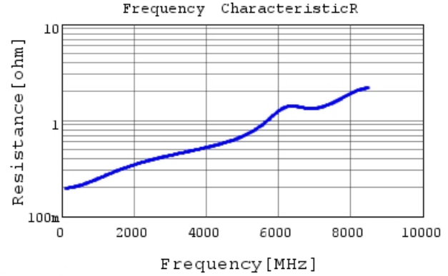
GRM1555C1H8R0CA01 R DCOV, 25degC
