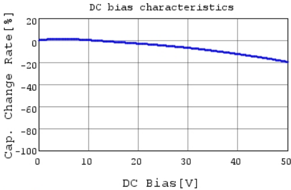
GCM155R71H681KA37 C-DC bias capchange, 25.0c
