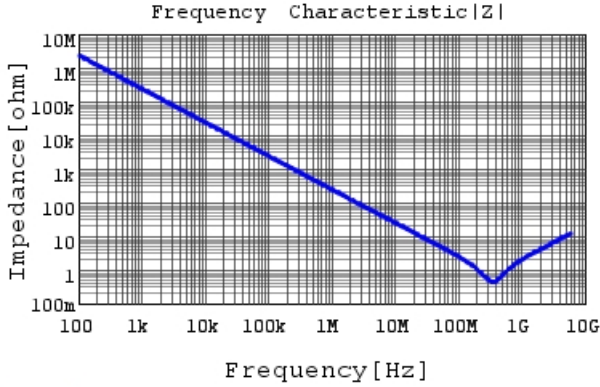
GCM155R71H681KA37 |Z| DCOV, 25degC
