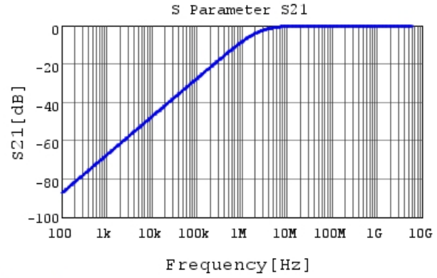
GCM155R71H681KA37 S21 DC0V, 25degC
