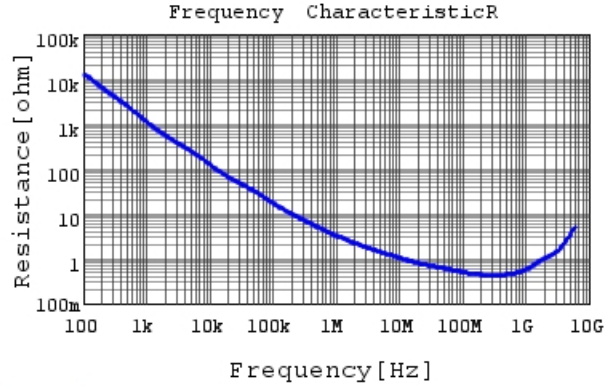
GCM155R71H681KA37 R DCOV, 25degC
