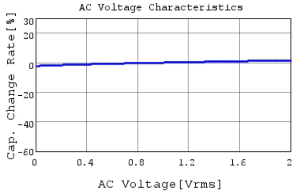
GCM155R71H681KA37 C-AC Voltage capchange, Dc
