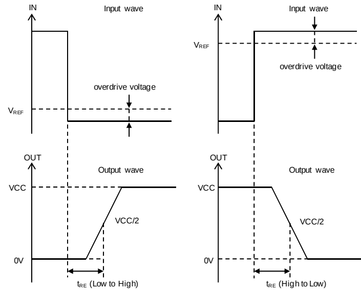
Figure 51. Response Time
