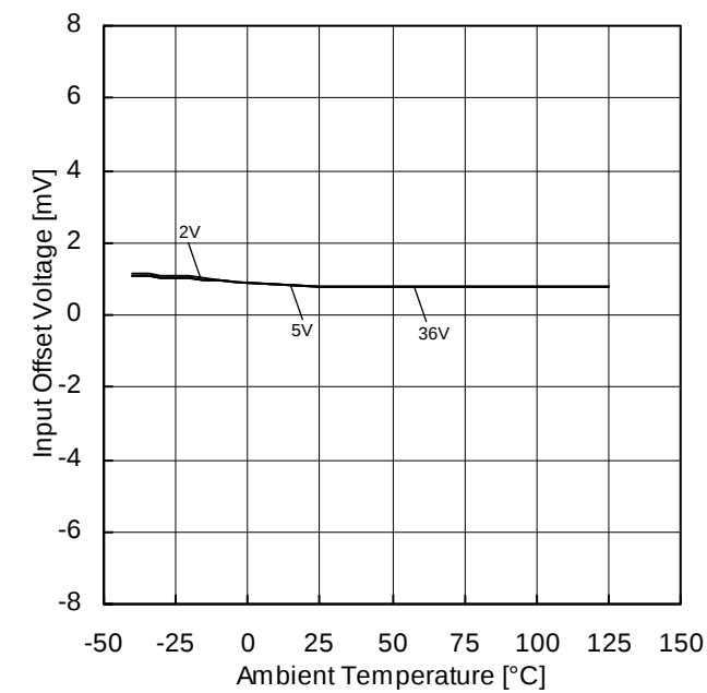
Figure 33. Input Offset Voltage vs Ambient Temperature
