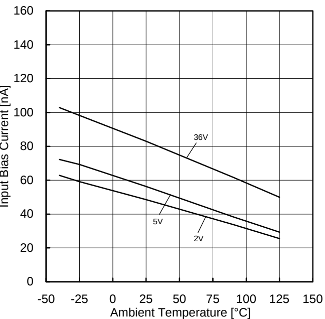
Figure 35. Input Bias Current vs Ambient Temperature
