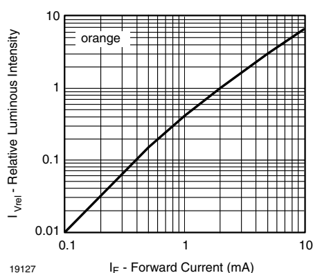
Fig. 14 - Relative Luminous Intensity vs. Forward Current
